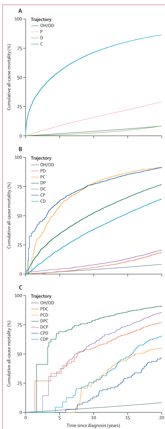
Figure 2: Cumulative all-cause mortality following diagnosis with one (A), two (B), or three (C) conditions for a 50-year-old man in the third quintile of the Welsh Index of Multiple Deprivation Diseases are referred to by their one-letter abbreviations, with the order of letters indicating the order in which the diseases were diagnosed within a trajectory. C=congestive heart failure. D=diabetes. OH/OD=otherwise healthy or otherwise diseased. P=psychosis.
